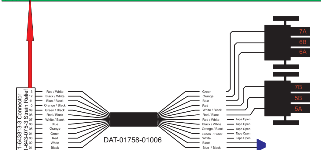
Viewed with Tyco Connector Plug-In Face-Down.
