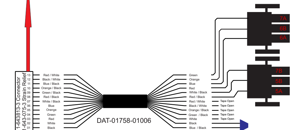
Viewed with Tyco Connector Plug-In Face-Down.
