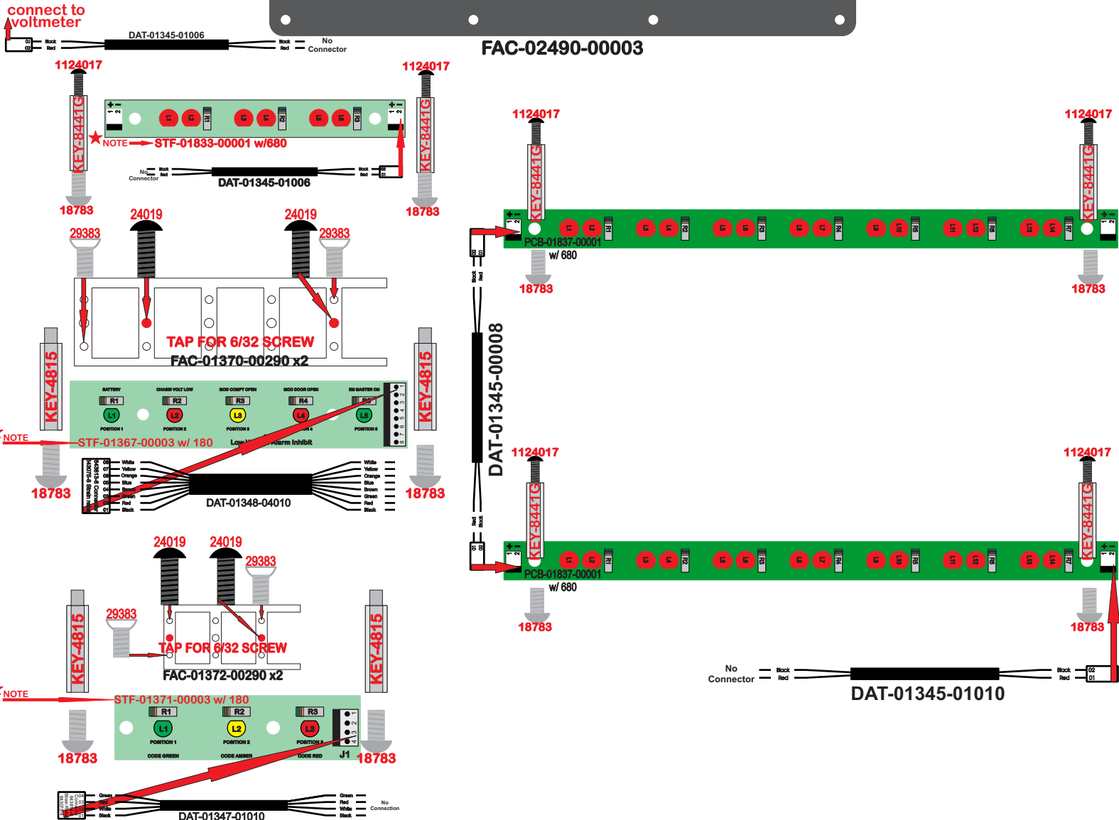
VOLTMETER DIGITAL RCT-02043-00000
