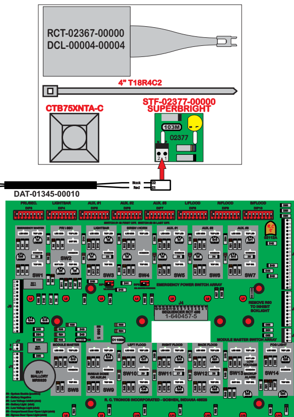
VIEW A RCT-02367 COMPLETE ASSY
