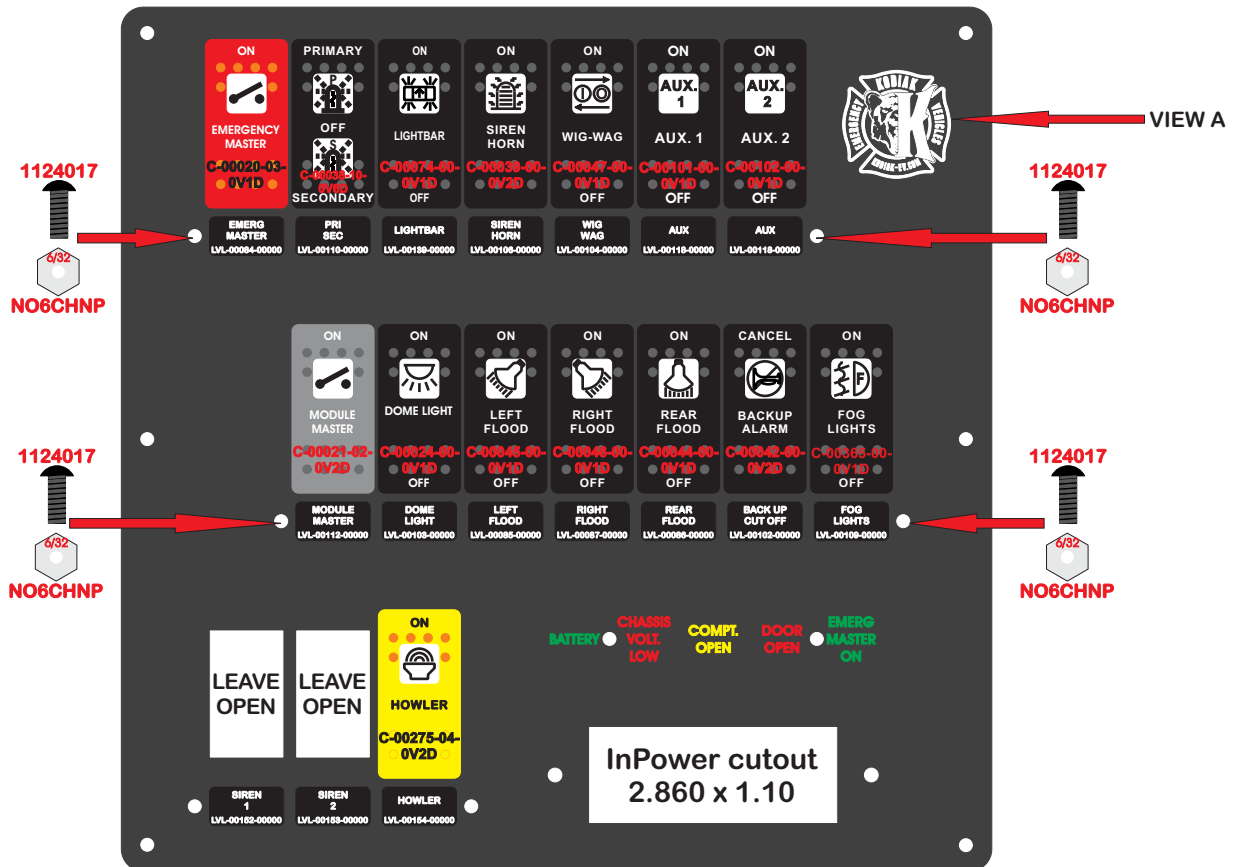
RTE-02804-00001 size 10.075 x 10 inches
