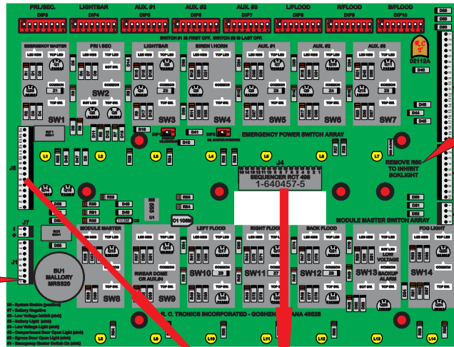
FAC-02807-00000 SIZE 12 X 10 INCHES
