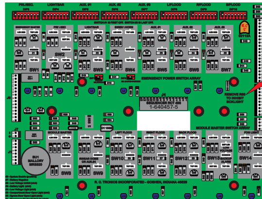
RCT-02367 COMPLETE ASSY
