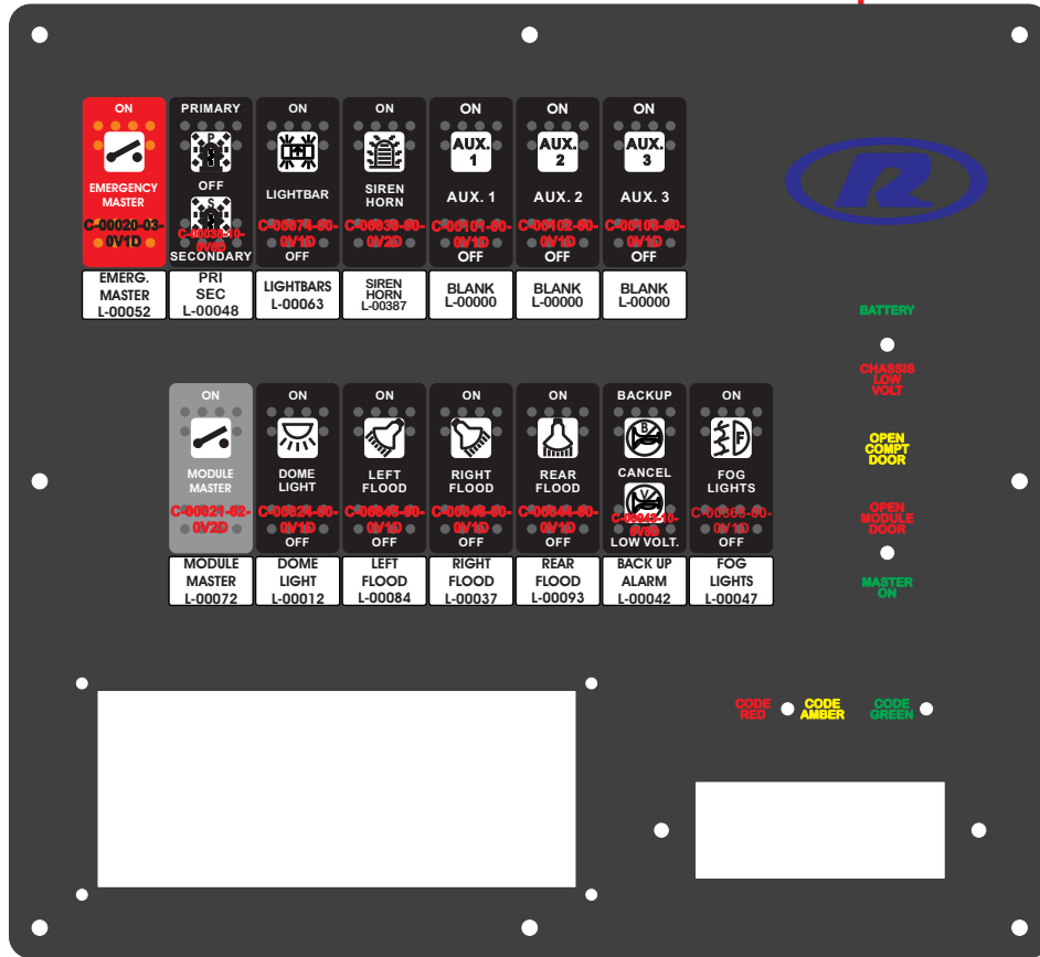
FAC-03225-0000 SIZE 12 X 11 INCHES
