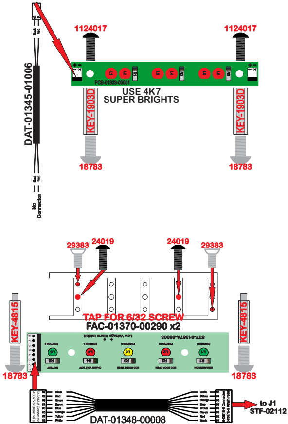
RTE-03281-00000 size 10.075 x 10 inches VIEW A RCT-02367 COMPLETE ASSY
