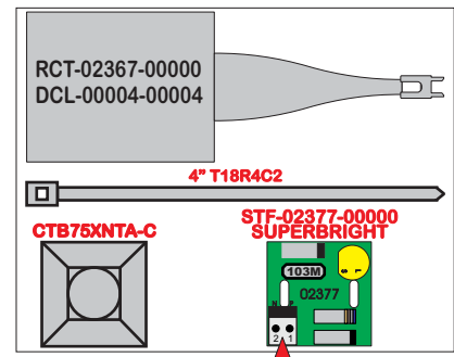
RTE-03281-00000 size 10.075 x 10 inches VIEW A RCT-02367 COMPLETE ASSY
