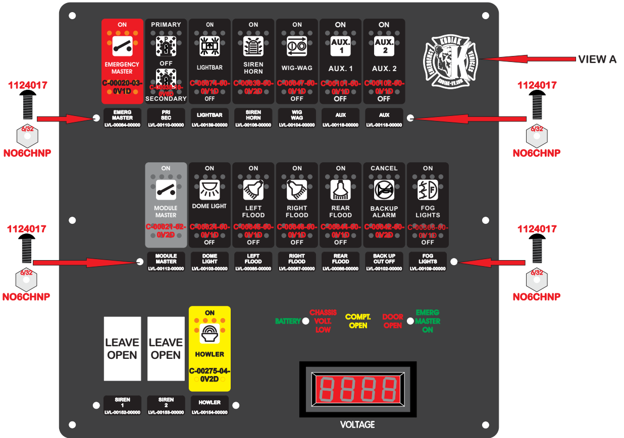
RTE-03281-00000 size 10.075 x 10 inches VIEW A RCT-02367 COMPLETE ASSY
