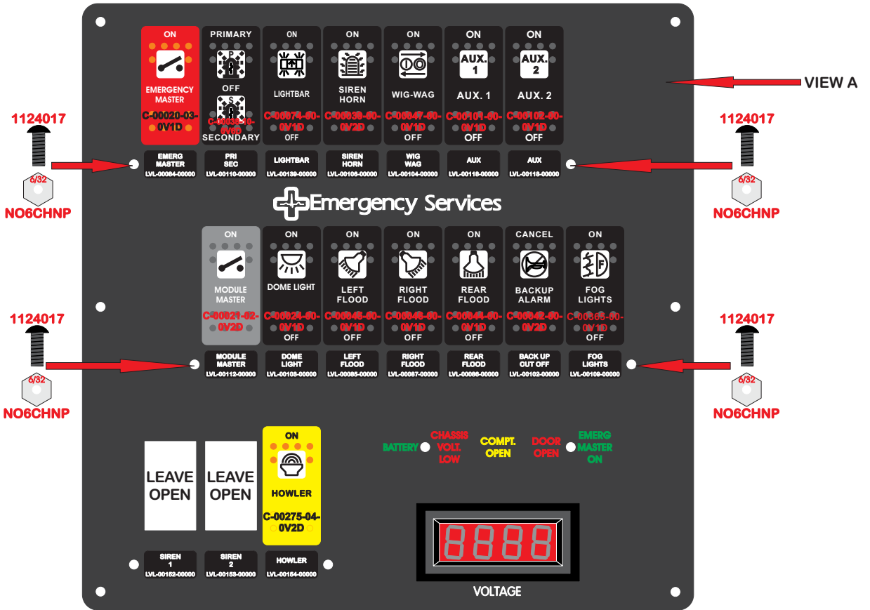
RTE-03281-00001 size 10.075 x 10 inches VIEW A RCT-02367 COMPLETE ASSY
