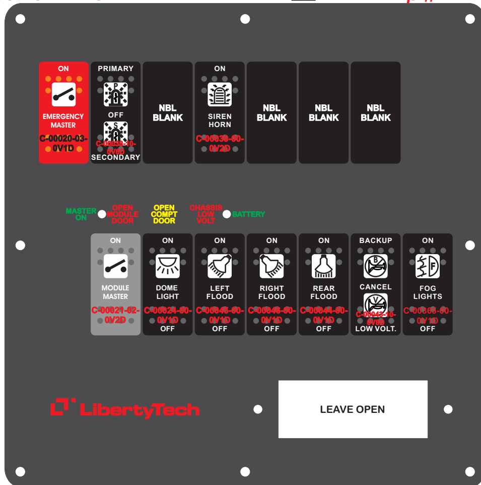
RCT-02366 COMPLETE ASSY
